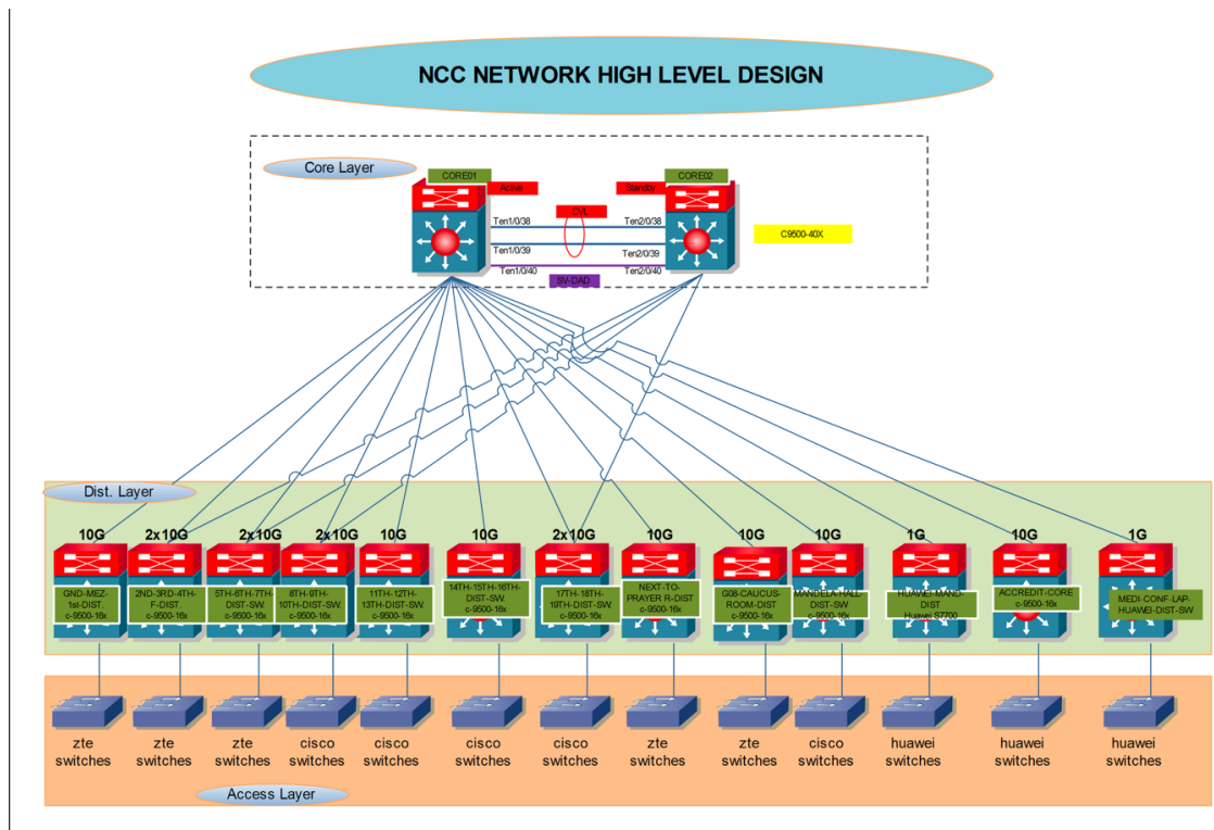
Figure 1. Current Logical Architecture for NCC Campus
