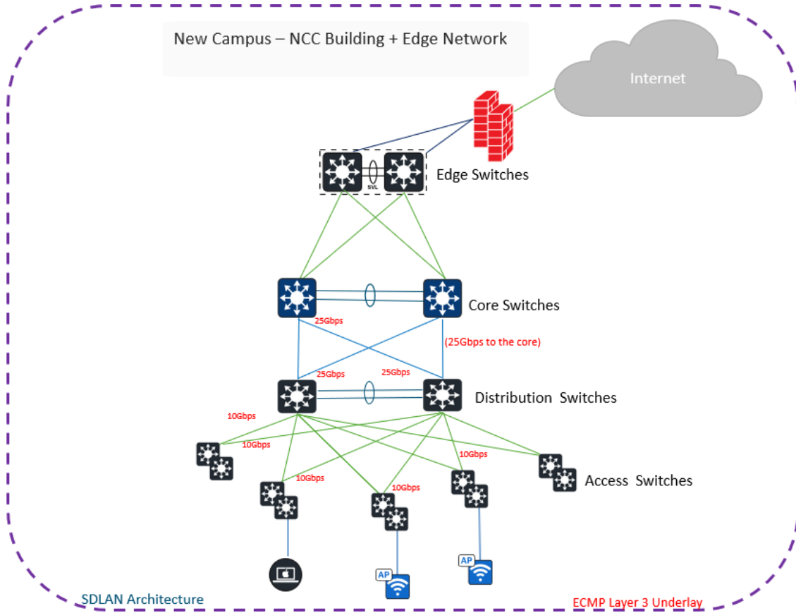
Figure 2 SD LAN Architecture – New Campus – NCC Building
