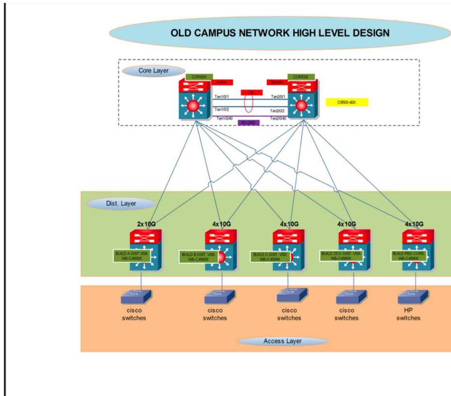
Figure 2. Current Logical Architecture for Old Campus.
