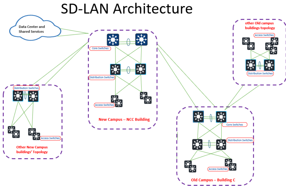
Figure 4 SD LAN overall envisioned Architecture
