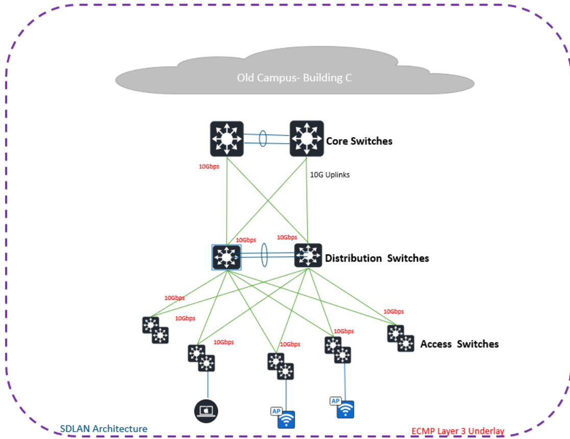
Figure 3 SD LAN Architecture – New Campus – NCC Building
